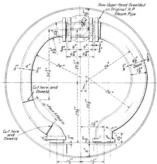
Fig. 4—Welded Steam Pipes for a Converted Cross-Compound Locomotive
